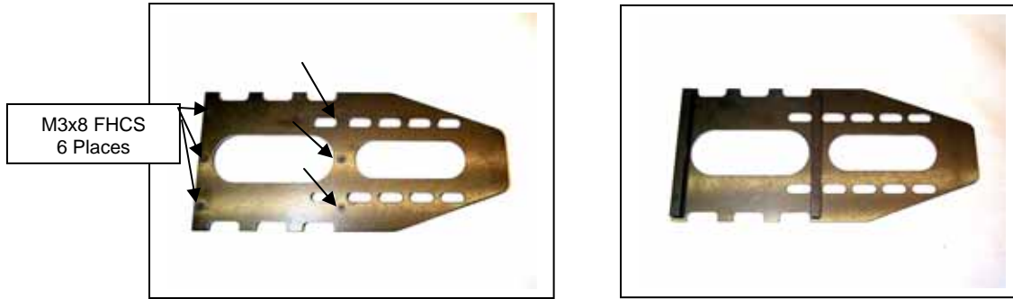
Bottom View Battery Tray, Countersink Holes Up
